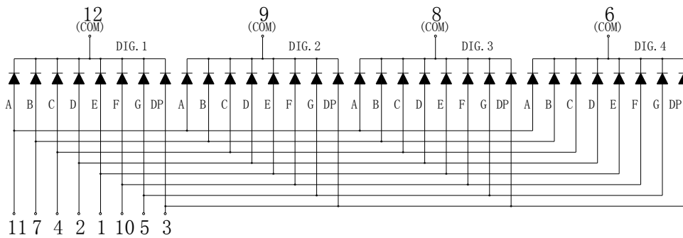
KW4-S391CVA
