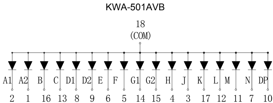
Internal Circuit Diagram (Common Anode)
