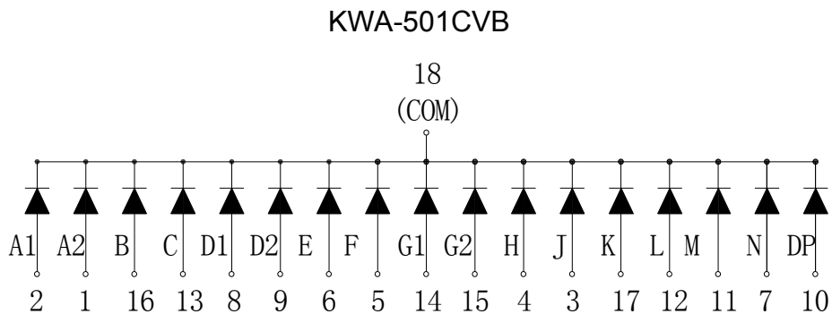
Internal Circuit Diagram (Common Cathode)
