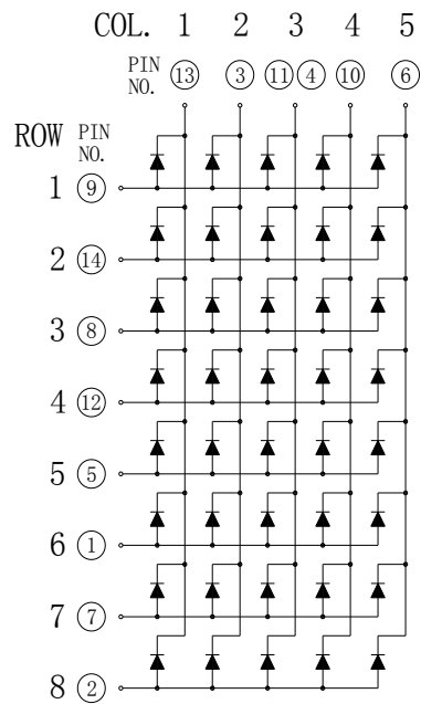
Common Row Anode: KWM-50581AWB
