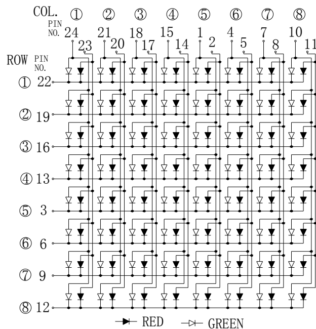
Common Row Cathode: KWM-50881CVPGB
