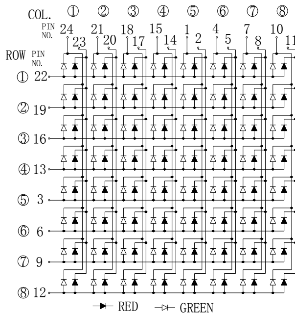
Common Row Anode: KWM-50881AVPGB
